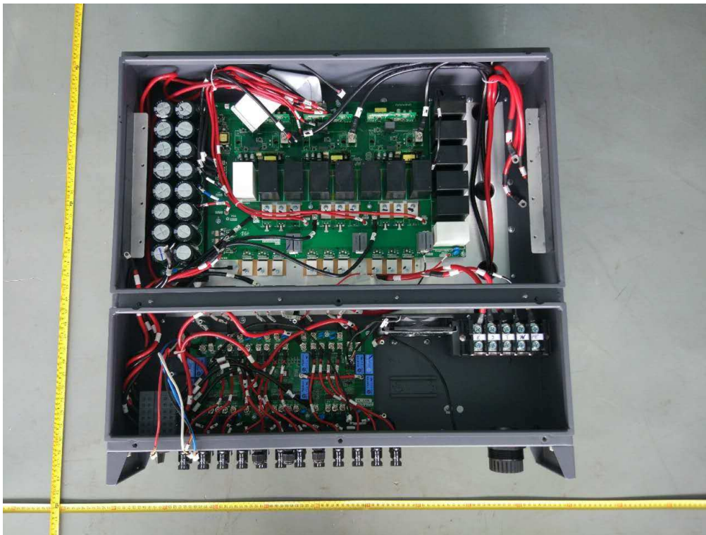
Internal view (EVVO 6000TL3P, EVVO 7000TL3P)
