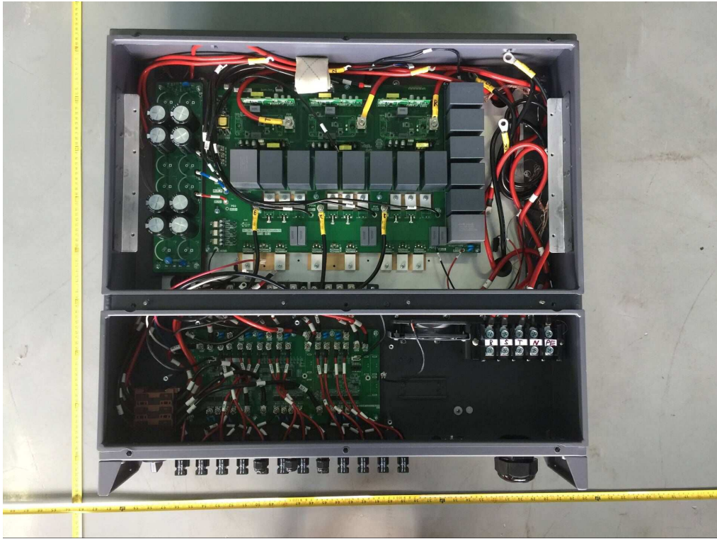
Internal view (EVVO 6000TL3P, EVVO 7000TL3P)
